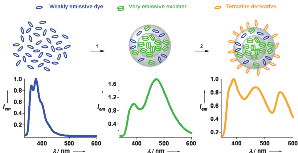
Figure 1. Representation of the co-grafting process: 1) formation of NPO; 2) Tz grafting reaction. Emission spectra ( \lambda_{\text{exc}} = 330 nm) of Napht (blue), NPO (green), and NPB (orange).
